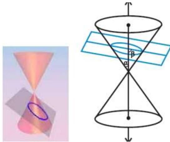
Ellipse
